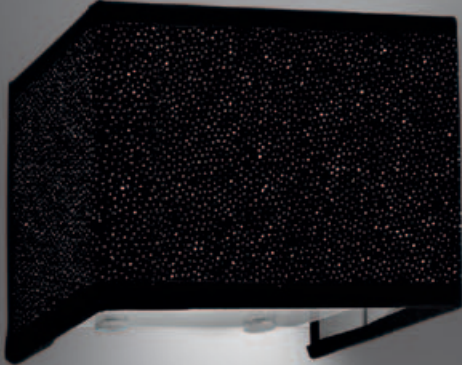
2769.01 L. 28 x 9 S. 8 cm. R7s 118mm.#1x100W oppure 2G11#1x18W 1 LED10W-300MA-Natural
